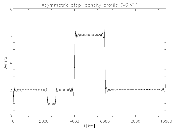
Fig. 5. Step density Profile: V_0, V_1(\delta_{min} = 0.41L^{-1}, \delta_{max} = 300L^{-1})
