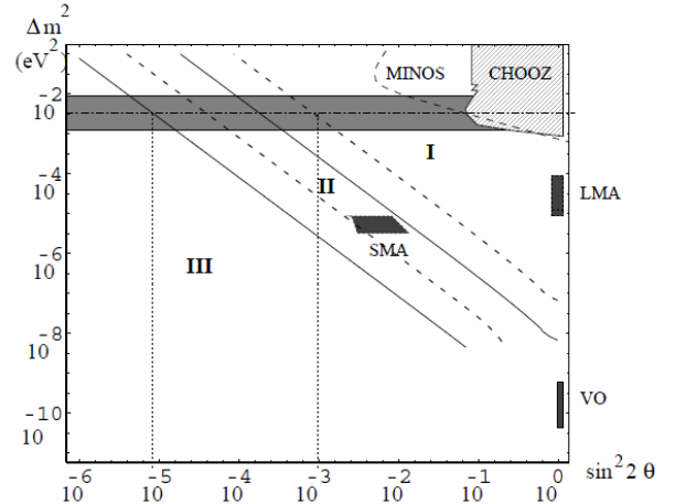
Fig. 2: Contours of equal P_f in the (\Delta m^2, \sin^2 2\theta) -plot for two different energies on the borders of the observable spectrum (Solid lines for 5 Mev, and dashed lines for 50 Mev). [8]
