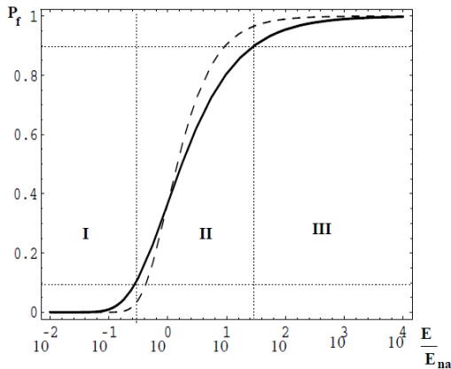
Fig. 1. the dependence of P_f on E/E_{na} (the solid line is for the density profile \rho \sim r^{-3} , and the dashed line is for a density profile \rho \sim e^{-r} ) [8]
