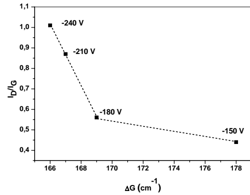
Figure 7: The ID/IG ratio plotted against the G peak FWHM for different values of V_b , as indicated.
