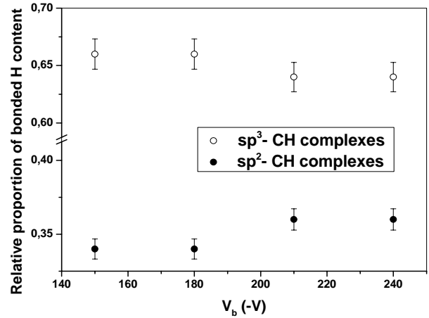
Figure 3: Variation of the relative proportion (%) of the H bonded as sp 3 -C-H and sp 2 -C-H complexes, as a function of V b
