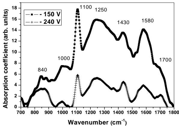
Figure 5: Typical FTIR spectra in the bending modes range for series I and IV.
