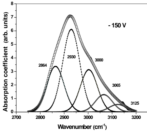
Figure 2: Example of decomposition of the stretching band into a sum of Gaussian contributions corresponding to the different vibration modes shown for sample of series I.
