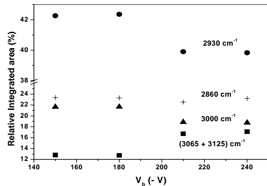
Figure 4: Variation of integrated area of the different Gaussian components that fitted the stretching IR absorption band, as a function of V b , as indicated.
