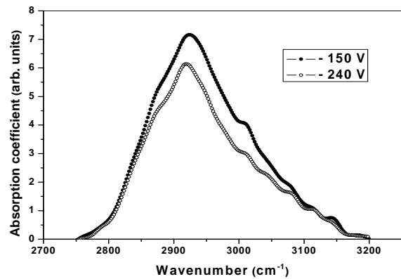
Figure 1: Typical FTIR spectra in the stretching modes range obtained for films deposited with V_b equal to -150 V and -240 V (samples of series I and IV, respectively).
